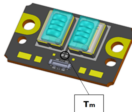
Figure 2. Temperature measurement point
